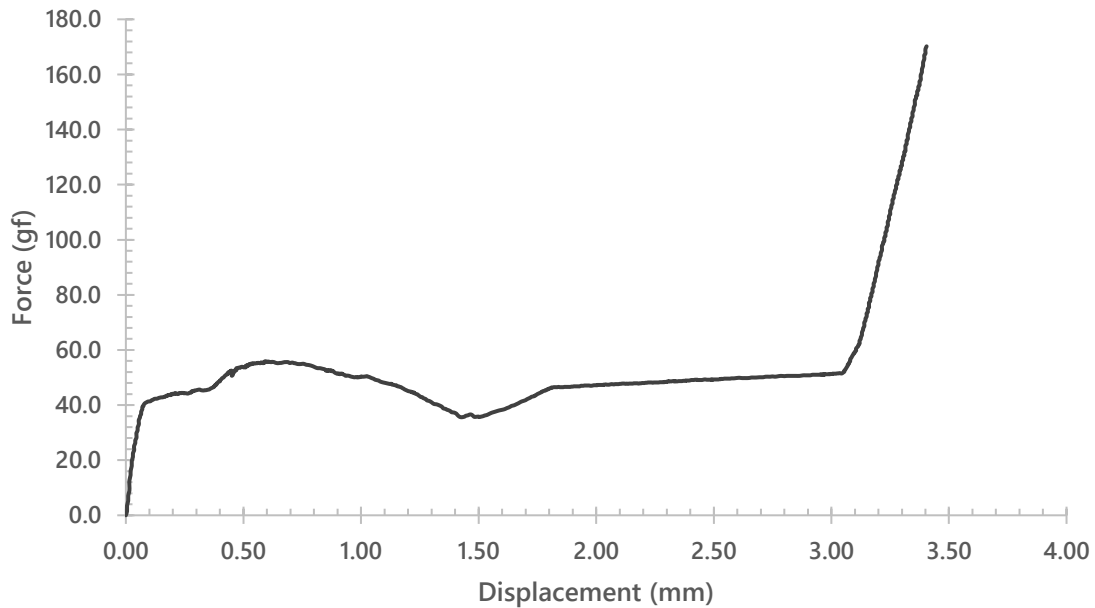
Gateron Milky Pro Purple (Upstroke)
